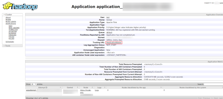
图 5-8 application
